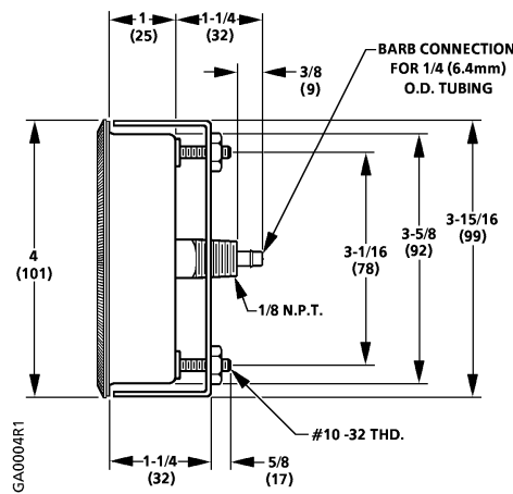
Figure 4. 3-1/2-Inch Gauge.
