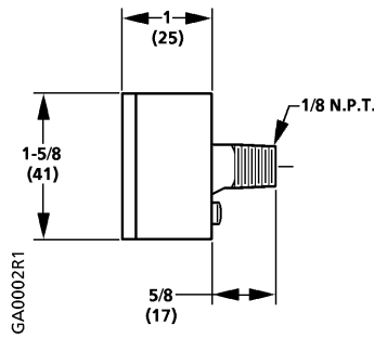
Figure 2. 1-1/2-Inch Gauge.
