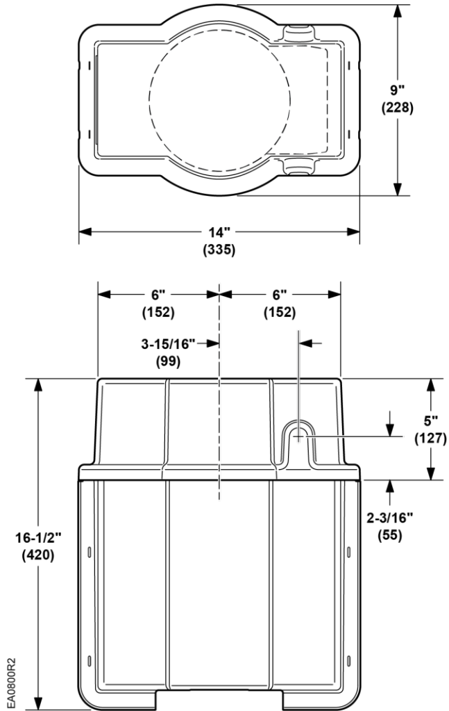
Figure 17. Dimensions of the 599-10065 Weather Shield in Inches (Millimeters).
