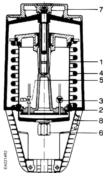
Figure 6. Actuator Design.
