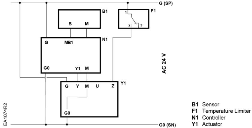
Figure 14. Connecting Terminals.
