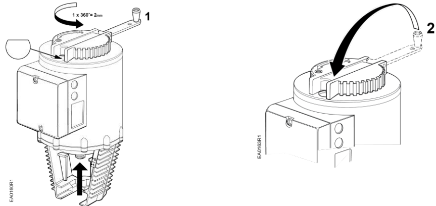
Figure 13. Automatic Operation.
