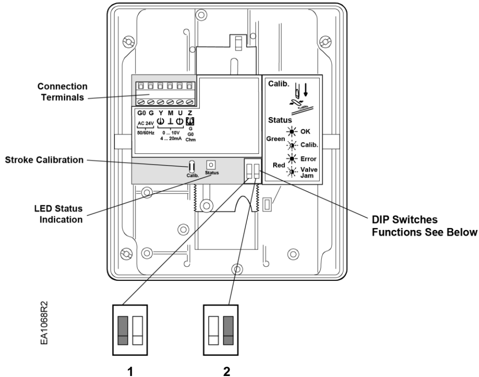
Figure 10. DIP Switches.
