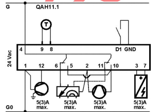
Figure 7. Heat Pump Wiring.
