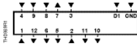
Figure 5. Wiring.
