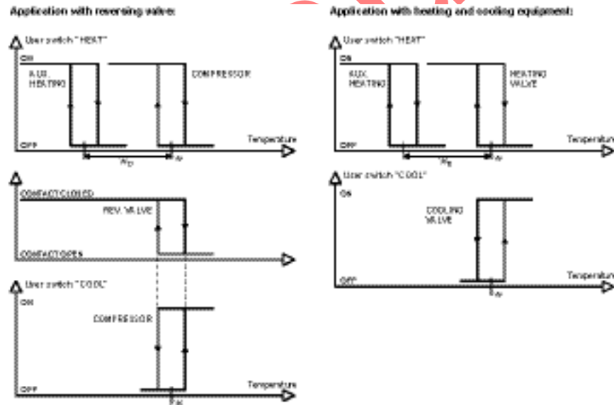
Figure 1. Operation Diagrams.
