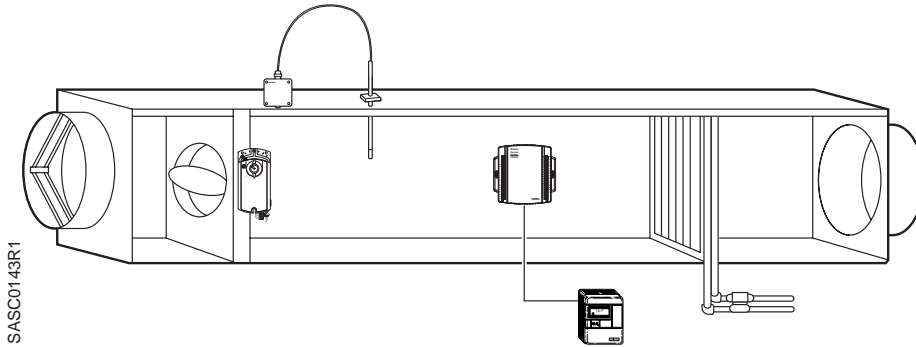
VAV with Reheat (HW or Electric)
