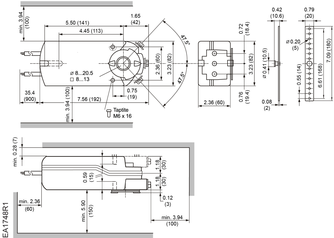
Figure 21. Dimensions of the GEB Actuator and Mounting Bracket in inches (mm).
