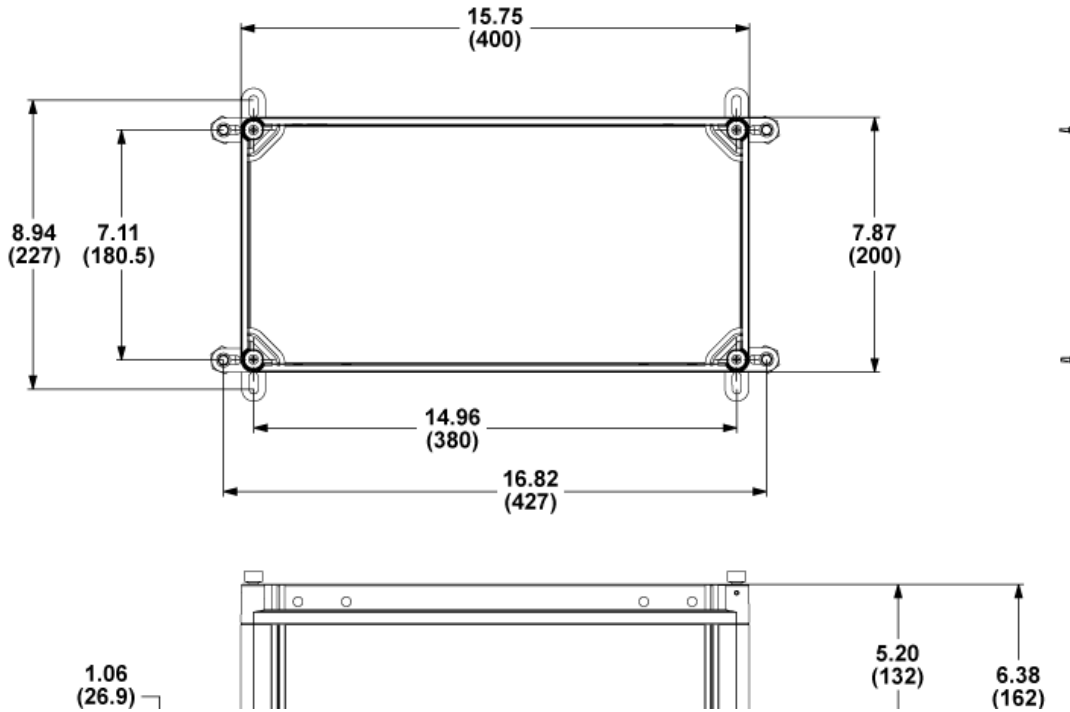
Figure 20. Dimensions of the ASK75.7U Weather Shield in Inches (Millimeters).
