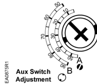
Figure 15. Dual Auxiliary Switch Dials.
