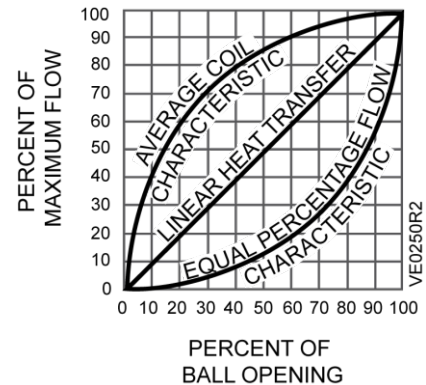
Figure 3. Ball Valve Equal Percentage Flow Control.
