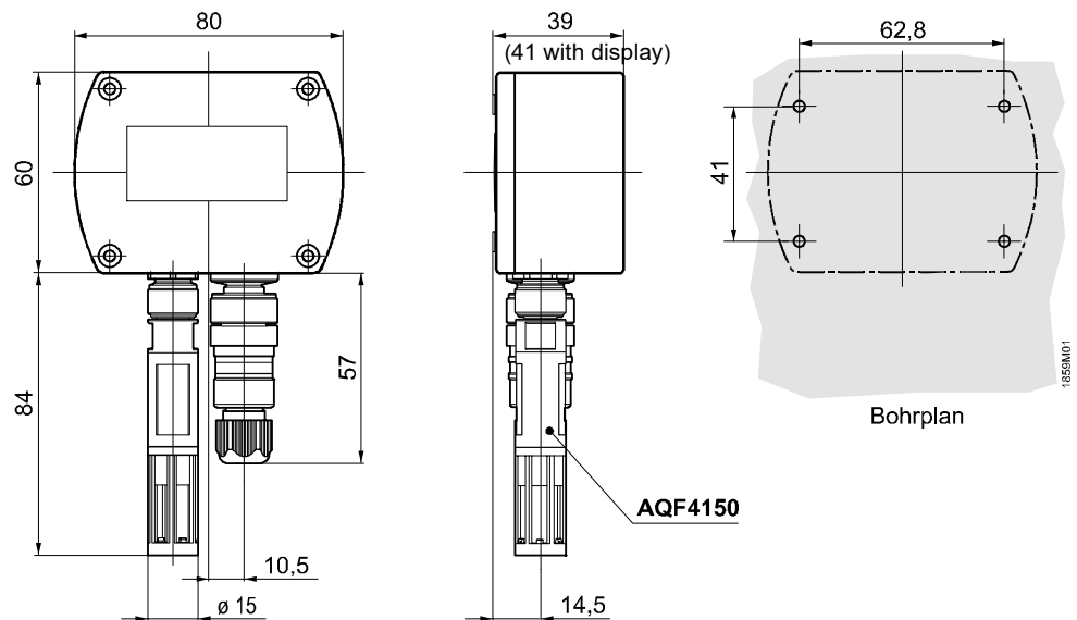
Dimensioning without (with) LCD-display Dimensions in mm
