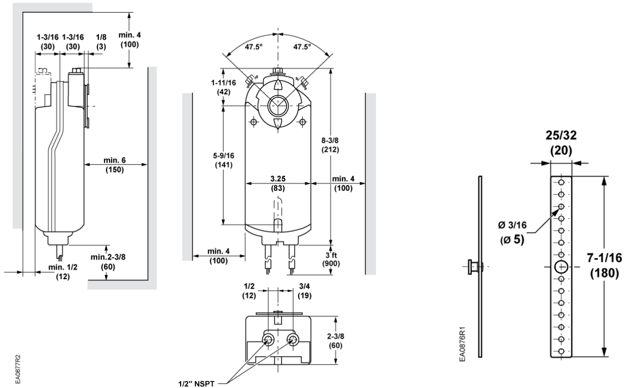
Figure 20. Dimensions of the GEB Actuator and Mounting Bracket in inches (mm).
