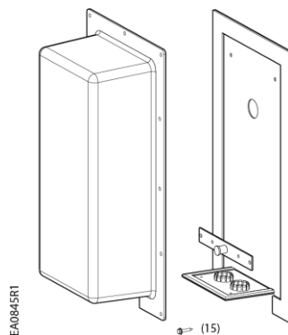
Figure 5. NEMA 3R Weather Shield.
