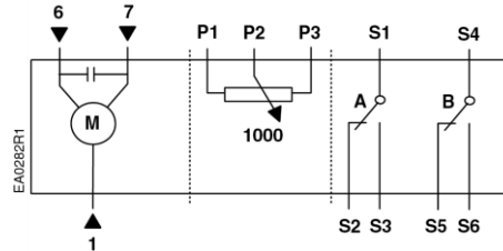
Figure 18. Floating Control. 24 Vac Power Supply.
