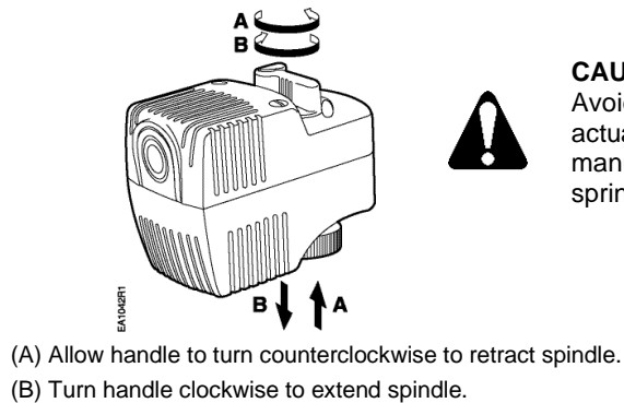
Figure 5. SFP Models, Normally Open.
