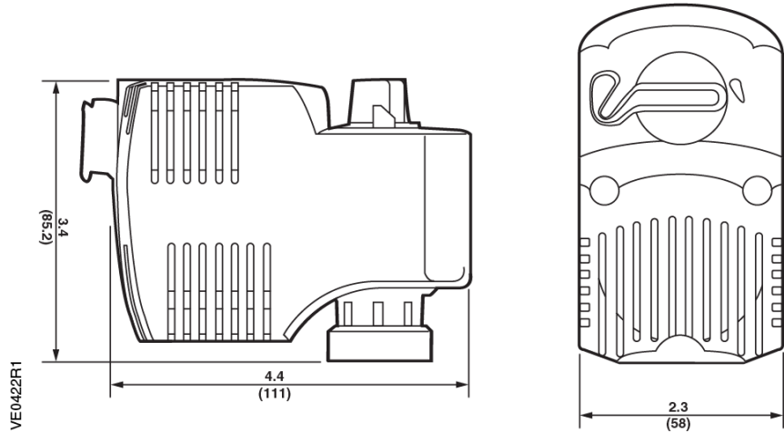
Figure 7. Dimensions of the SFx Series Actuator.
