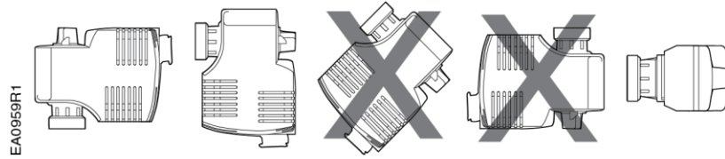
Figure 1. Mounting Position.
