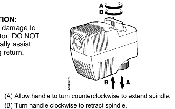
Figure 6. SFA Models, Normally Closed.
