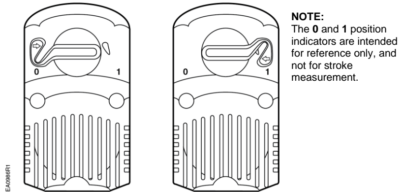
Figure 4. Manual Override Handle Positioning.
