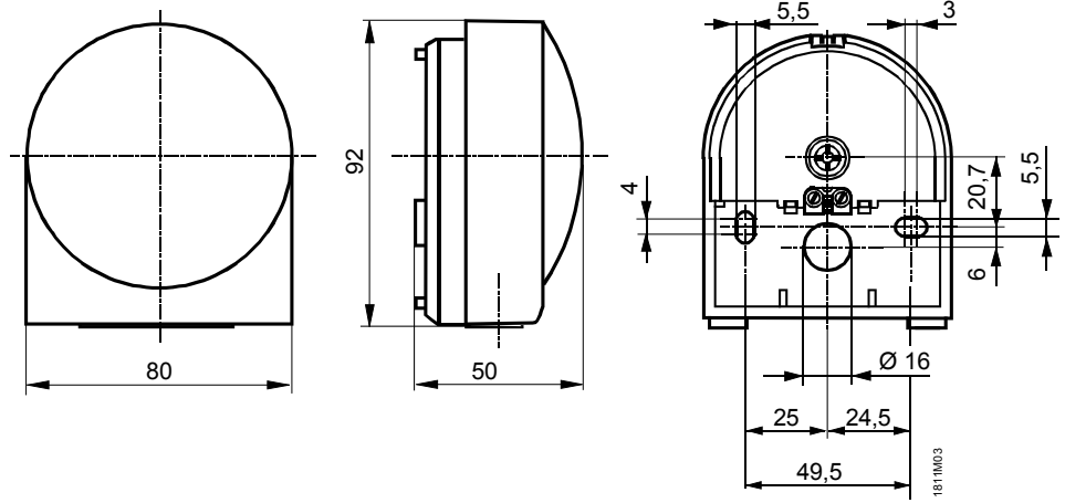
Drilling plan
