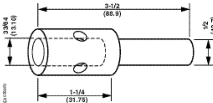
Figure 1. Dimensions in Inches (Millimeters).
