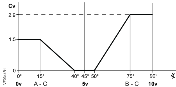
Figure 6. Example Control Characteristic Curve for 599-10601-1.5-2.9 and 171C-10601-1.5-2.9.
