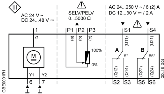
Figure 17. 24 Vac/Vdc 3-Position Control GEB14x.1U/1P.
