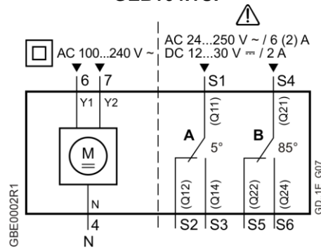
Figure 20. 100 to 240 Vac 3-position control GEB341.1U.
