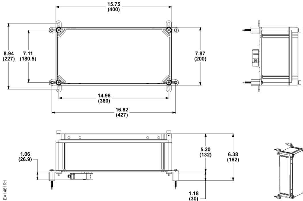
Figure 22. Dimensions of the ASK75.7U Weather Shield in Inches (Millimeters).
