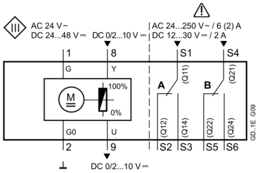
Figure 19. 24 Vac/Vdc Continuous control 0 to 10V GEB16x.1U/1P.
