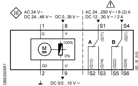
Figure 18. 24 Vac/Vdc Modulating Control DC 0 to 10V GEB164.1U.
