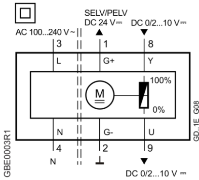
Figure 21. 100 to 240 Vac Modulating control DC 0 to 10V GEB361.1U.
