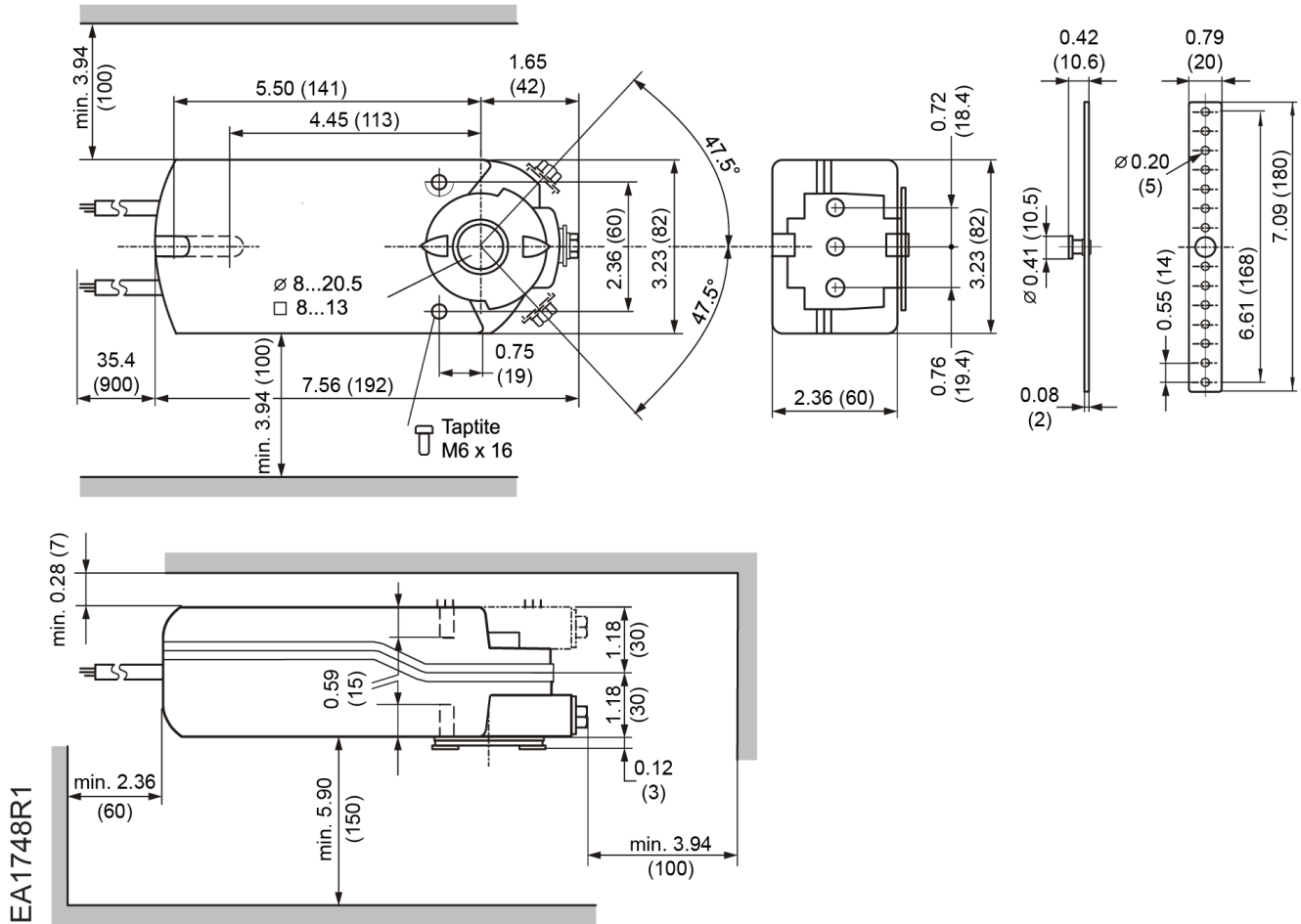
Figure 23. Dimensions of the GEB Actuator and Mounting Bracket in inches (mm).
