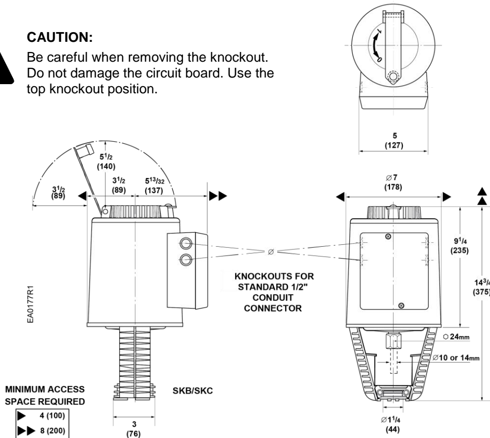
Figure 29. SKB/C62UA Dimensions in Inches (Millimeters).
