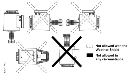
Figure 1. Acceptable Mounting Positions.
