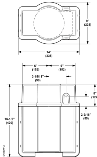
Figure 28. SKB/C Weather Shield, 599-10065 Dimensions in Inches (Millimeters).
