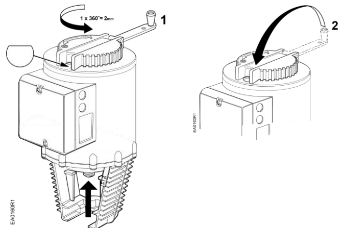
Figure 26. Return to Automatic Operation.
