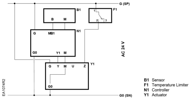
Figure 24. Wiring Diagram.
