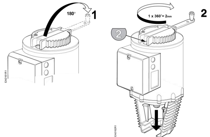
Figure 25. Manual Operation.
