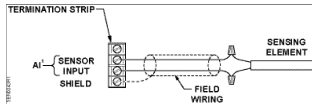
Figure 4. Typical Sensor Connection.
