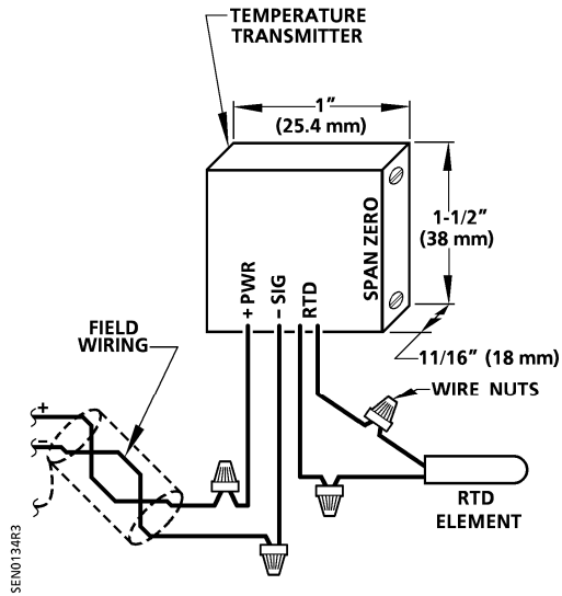
Figure 5. 536-780 (4 to 20 mA Output) Only.
