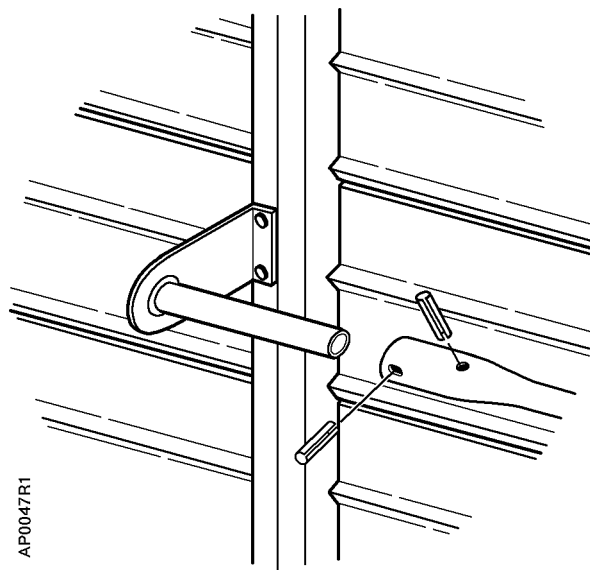
Figure 1. Installing the Damper Shaft Extension.
